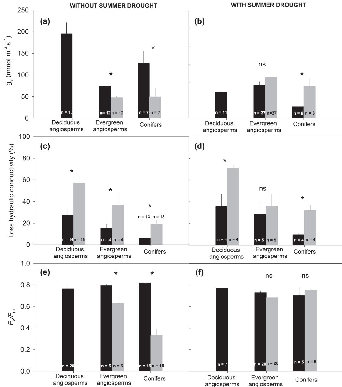
Figure 1. Results of a meta-analysis of shifts in leaf and stem physiology between summer and winter for woody species across the temperate zone, including mean values ( \pm SE) for (a, b) stomatal conductance ( g_s , mmol m -2 s -1 ), (c, d) percent loss of hydraulic conductivity (PLC) and (e, f) photochemical efficiency of photosystem II ( F_v/F_m ) during summer (black bars) and winter (grey bars) for deciduous angiosperms, evergreen angiosperms and conifers at sites without summer drought (a, c, e) and with summer drought (b, d, f). Asterisks (*) indicate significant differences ( p < 0.05 ) between sites summer and winter within each functional type. The number of species used for each functional type (n) is indicated at the base of each bar.
