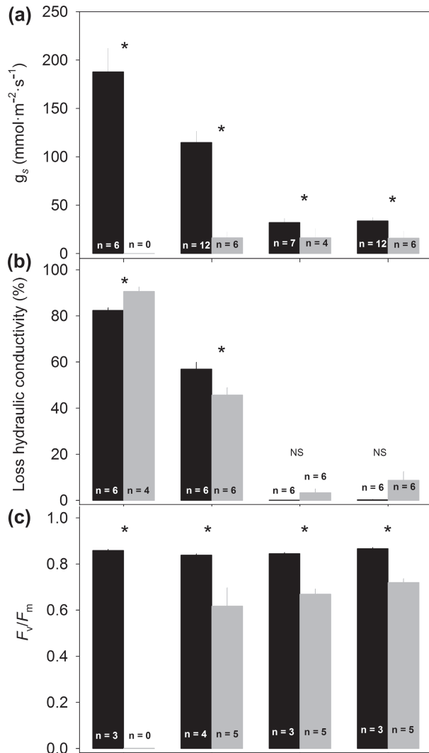
Figure 2. Shifts in leaf and stem physiology between summer and winter for four common, coexisting species in central Spain, including mean values ( \pm SE) for (a) stomatal conductance ( g_s , mmol m -2 s -1 ), (b) percent loss of hydraulic conductivity (PLC) and (c) photochemical efficiency of photosystem II ( F_v/F_m ) for the study species – Quercus faginea (winter deciduous angiosperm), Quercus ilex (evergreen angiosperm), Juniperus thurifera and Pinus nigra (conifers) – during summer (black bars) and winter (grey bars). Asterisks (*) indicate significant differences ( p < 0.05 ) between summer and winter within each species. The number of individuals per measurement (n) is indicated at the bottom of each bar.
